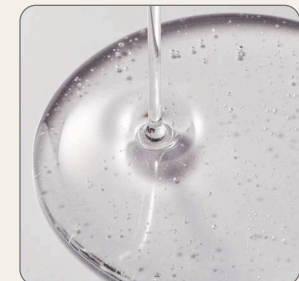
Hyaluronic Acid
