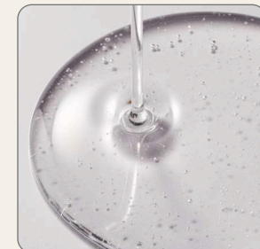
Hyaluronic Acid
